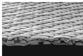
Double-layer fabric
